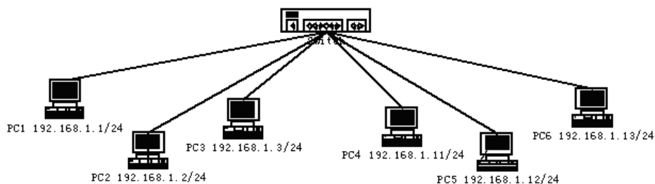
Figure 9 SuperVLAN
