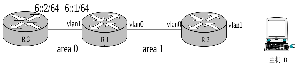
Figure 1.1 MCE in the MPLS-VRF VPN network
